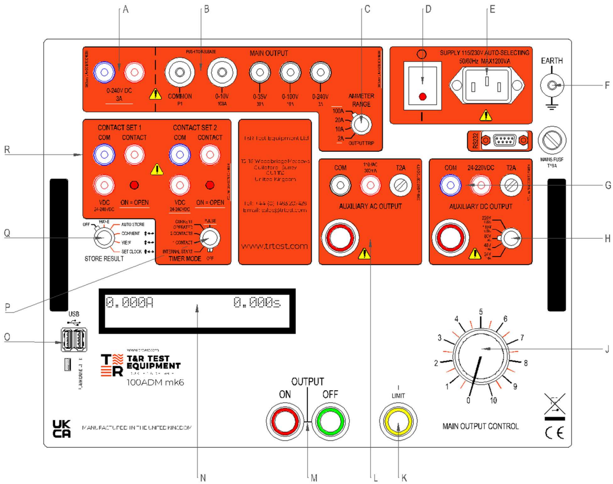
Figure 1.1 100ADM mk6 front panel
