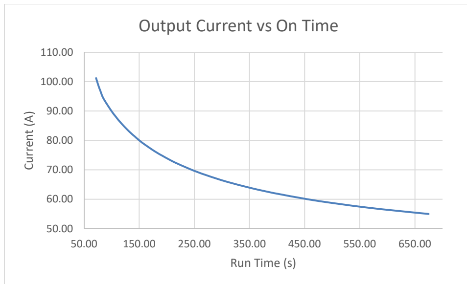
Figure 1.7 100ADM mk6 maximum 'on' times
