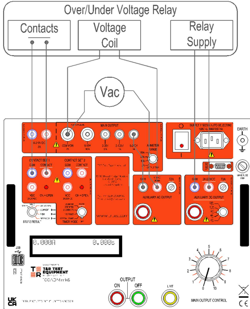
Figure 2.5 Voltage step
