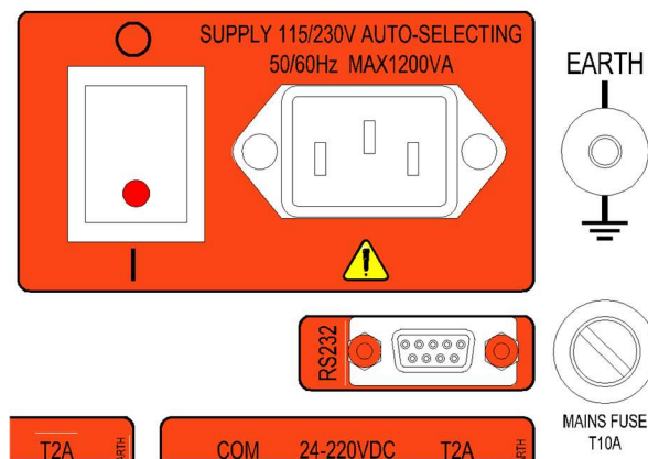
Figure 1.6 Mains input
