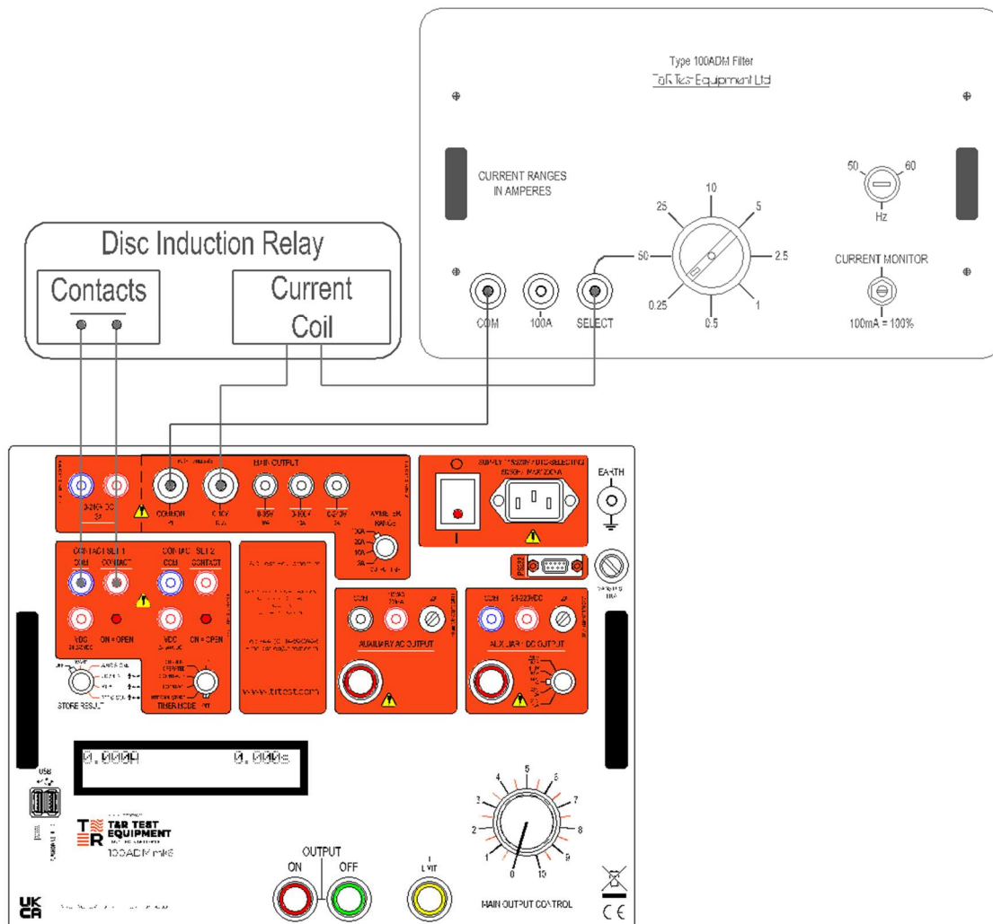
Figure 3.11 Connection of filter unit and inductive disc relay
