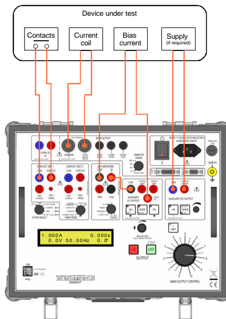
Figure 2.5 2 ac currents
