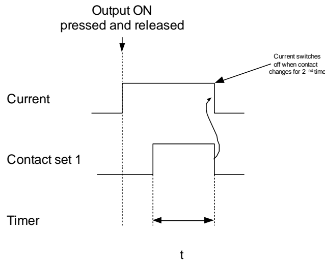
Figure 1.14 1 contact mode using contact set 2 (C2)
