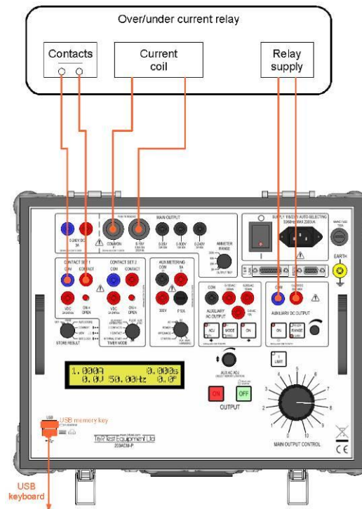
Figure 3.3 Connections for overcurrent timing
