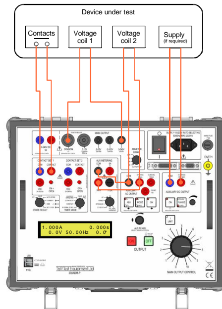
Figure 2.9 Two ac voltages
