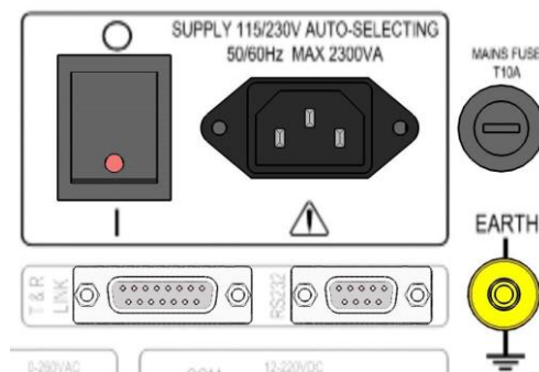
Figure 1.6 Mains input
