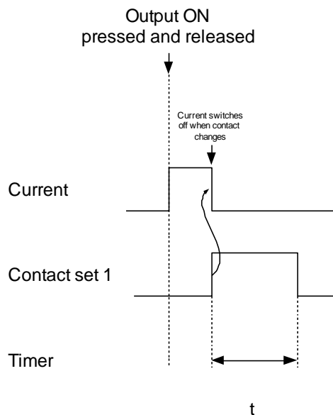
Figure 1.13 1 contact mode using contact set 1 (C1)
