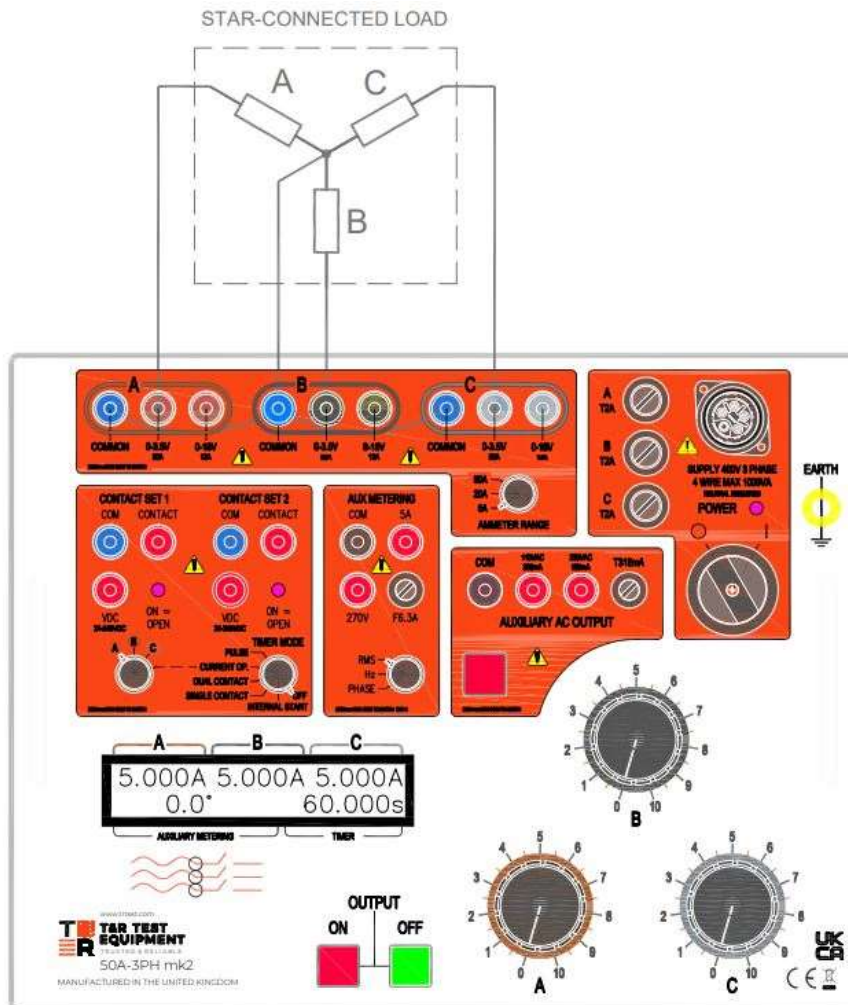
Figure 2.3 Connections for star-connected load
