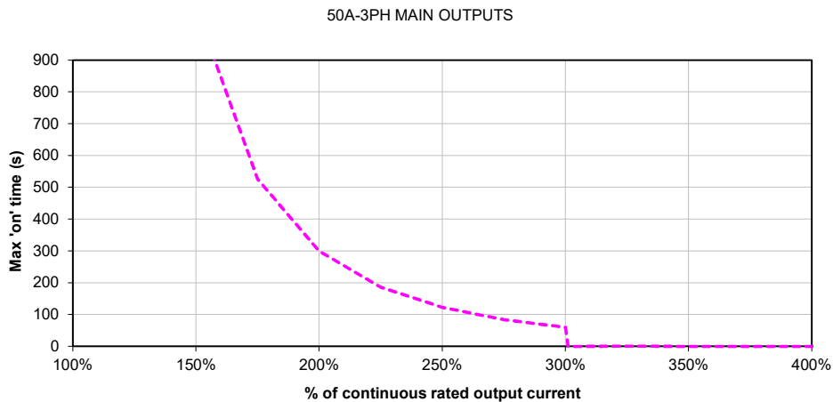
Figure 1.1 50A-3PH mk2 maximum 'on' times
