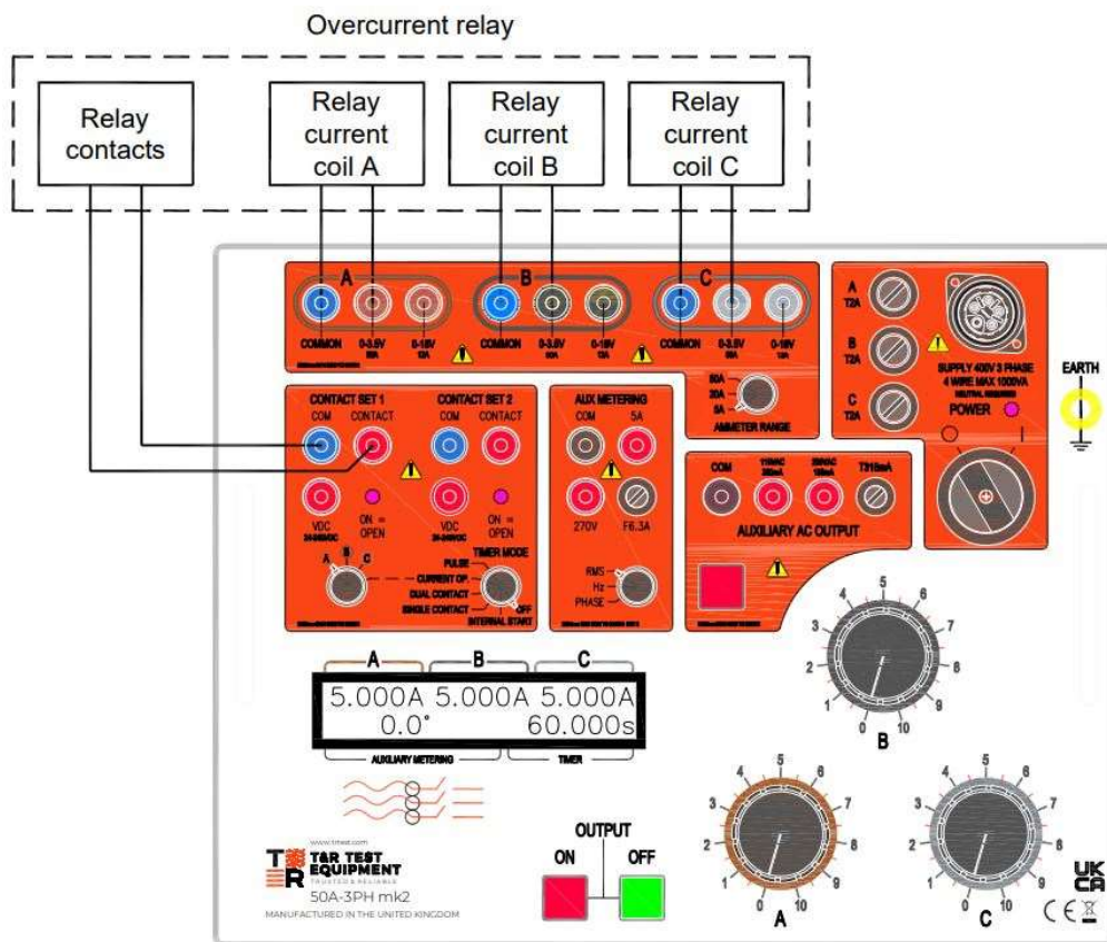
Figure 3.1 Connections for testing over-current relays
