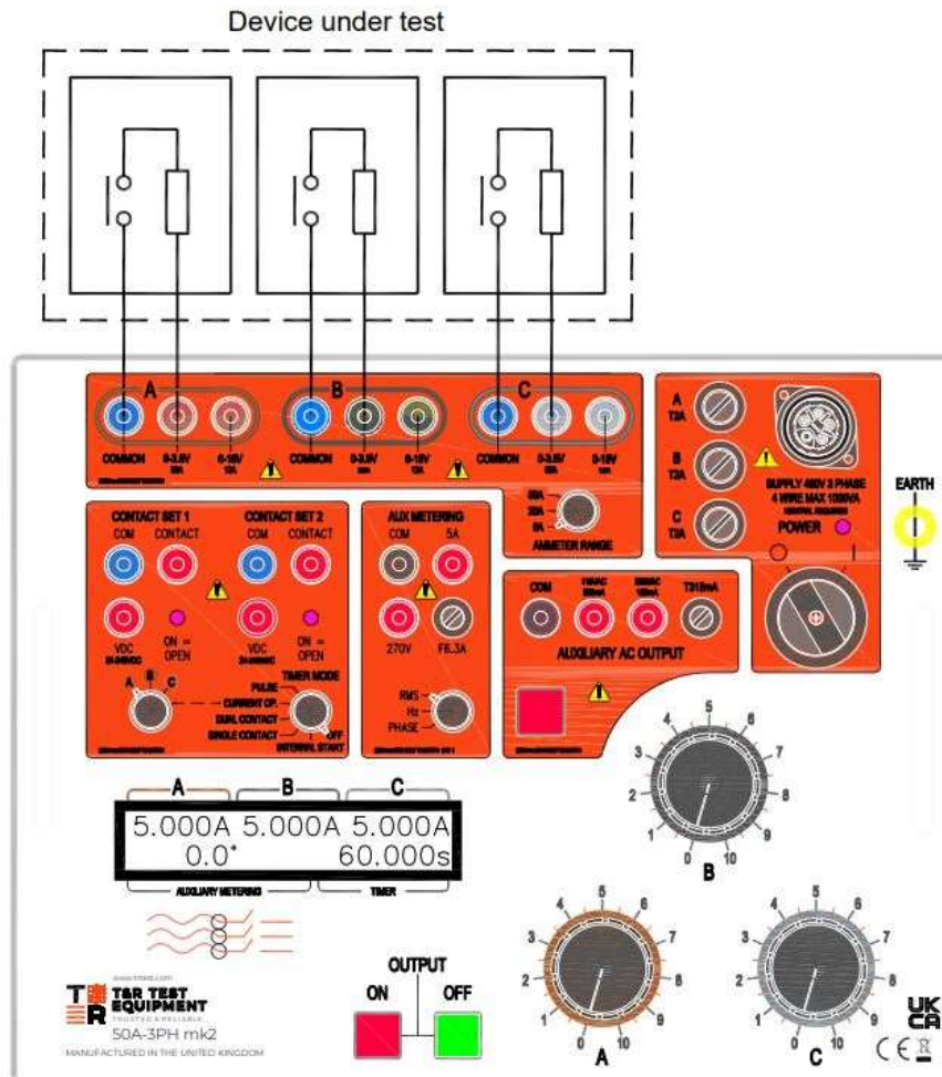
Figure 3.3 Connections for testing circuit breakers
