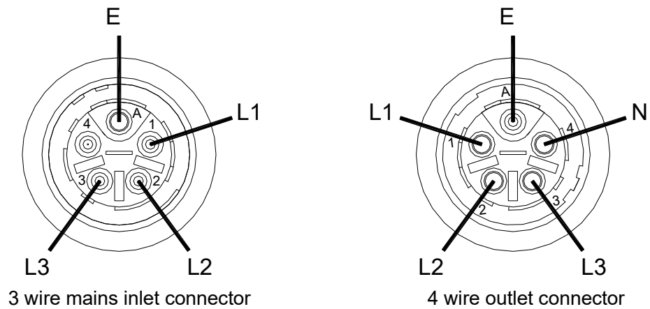
Figure 6.2 Mains inlet and three phase output connectors
