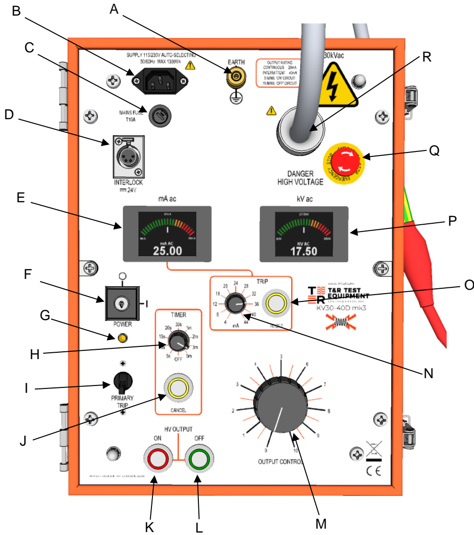
Figure 1.1 KV30-40D mk3 front panel
